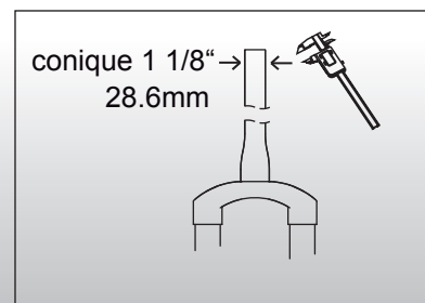
Fourche standard conique (tapered)
